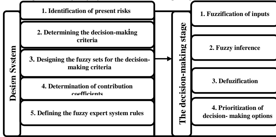
Fig. 3. Fuzzy risk assessment system.
