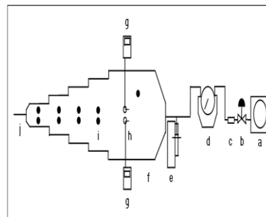
Fig.1: The schematic of the sampling set
